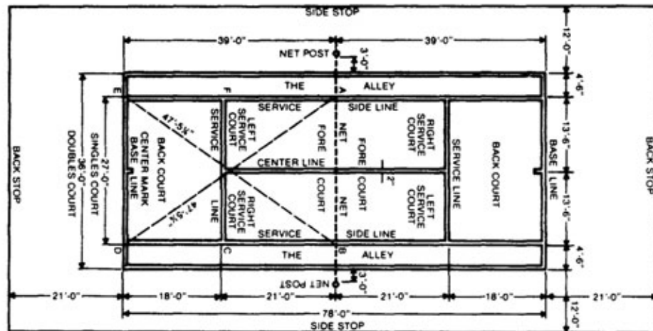
DOUBLES COURT LAYOUT
