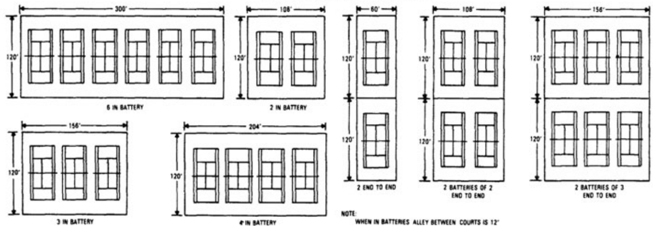
MULTIPLE COURT LAYOUT
