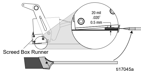
Screed Box
